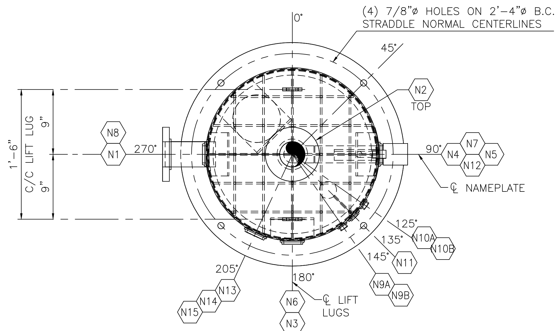
PLAN VIEW SCALE 1 1/2" = 1'-0" (TRUE ORIENTATION)
