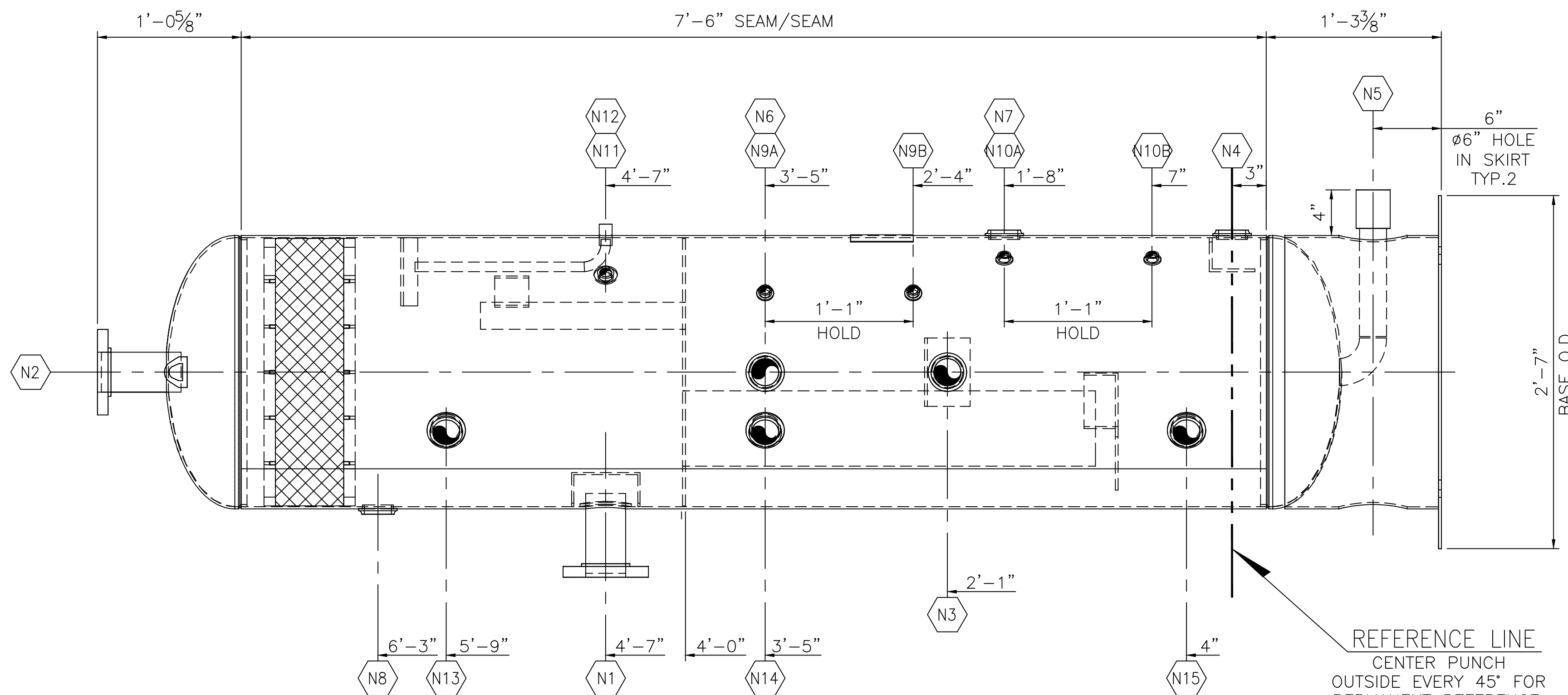
ELEVATION VIEW SCALE 1 1/2" = 1'-0"
