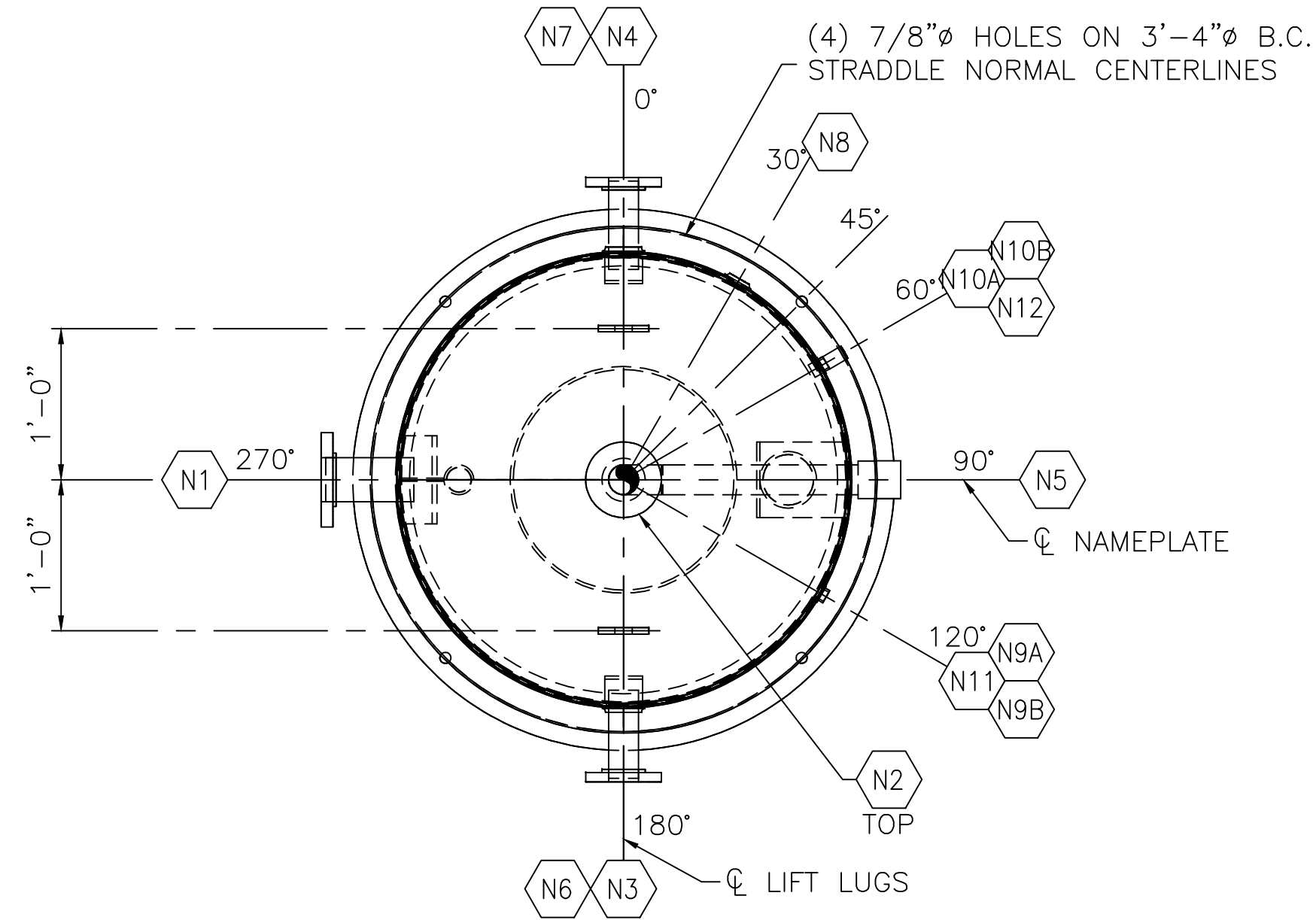
PLAN VIEW SCALE: 1" = 1'-0" (TRUE ORIENTATION)
