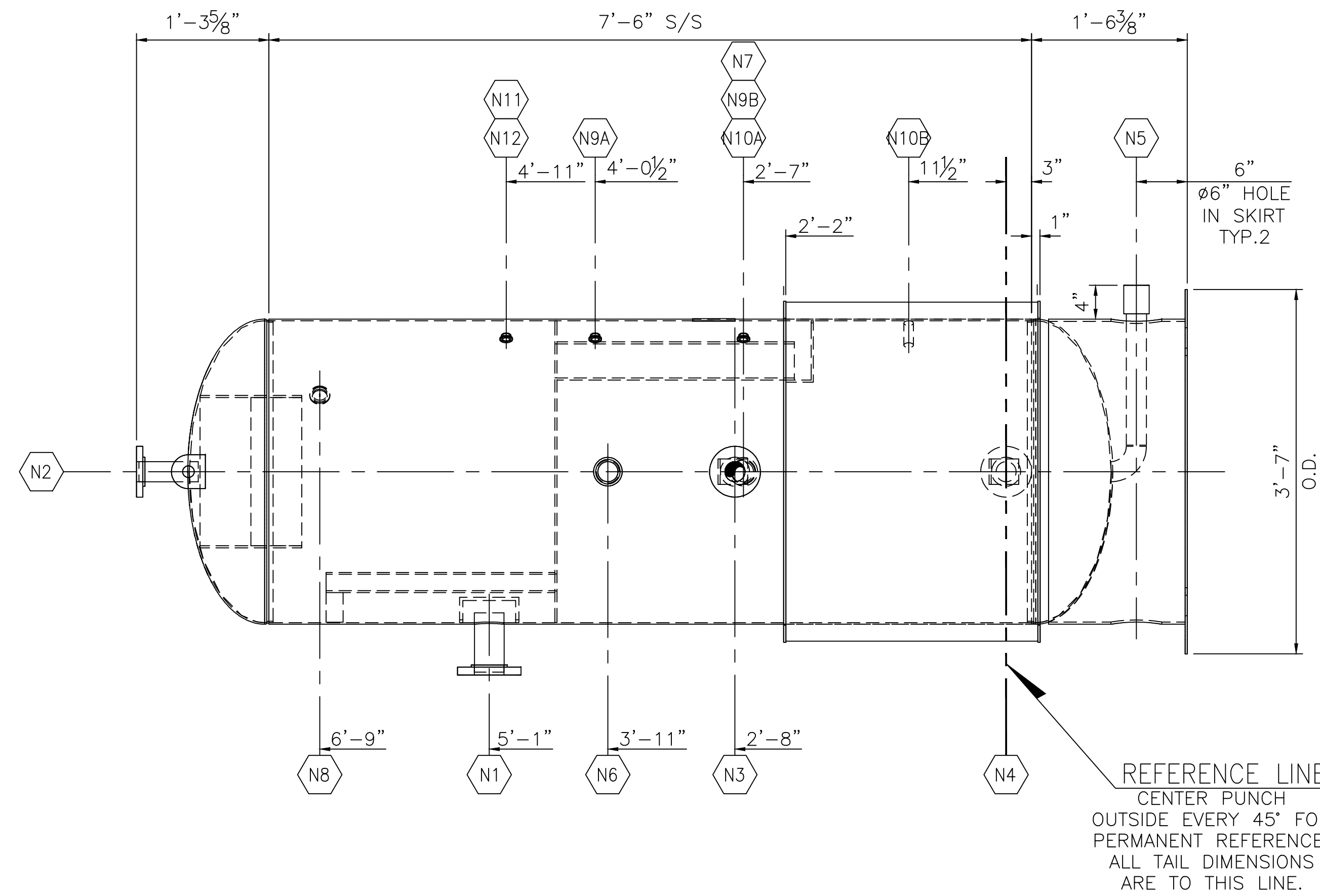
ELEVATION VIEW SCALE 1" = 1'-0"
