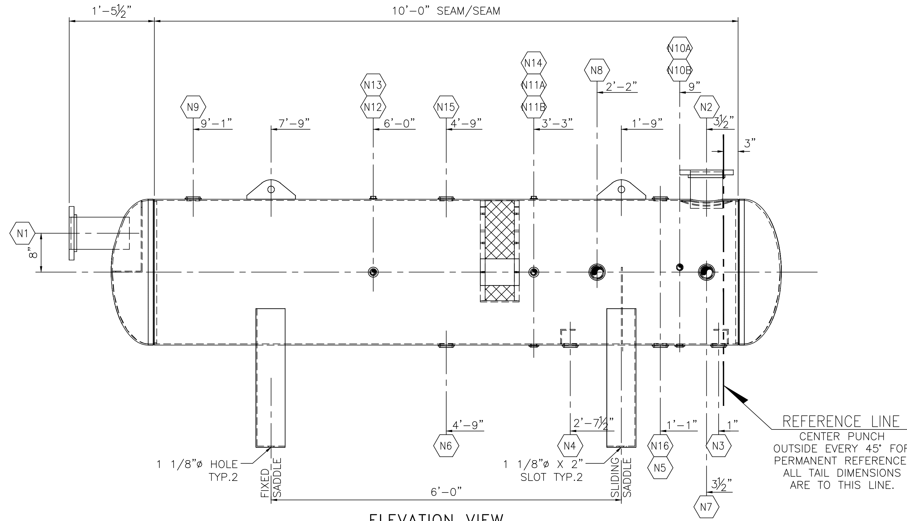
ELEVATION VIEW SCALE 1" = 1'-0"
