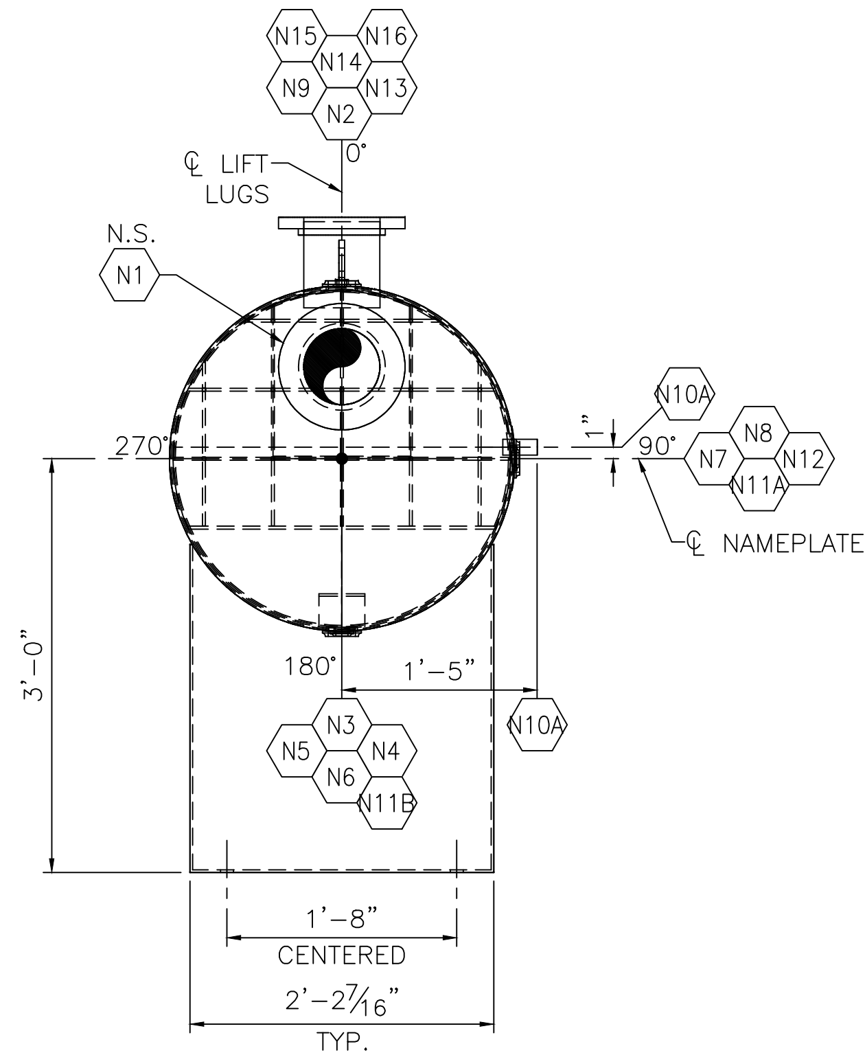
LEFT END VIEW SCALE 1" = 1'-0" (TRUE ORIENTATION)
