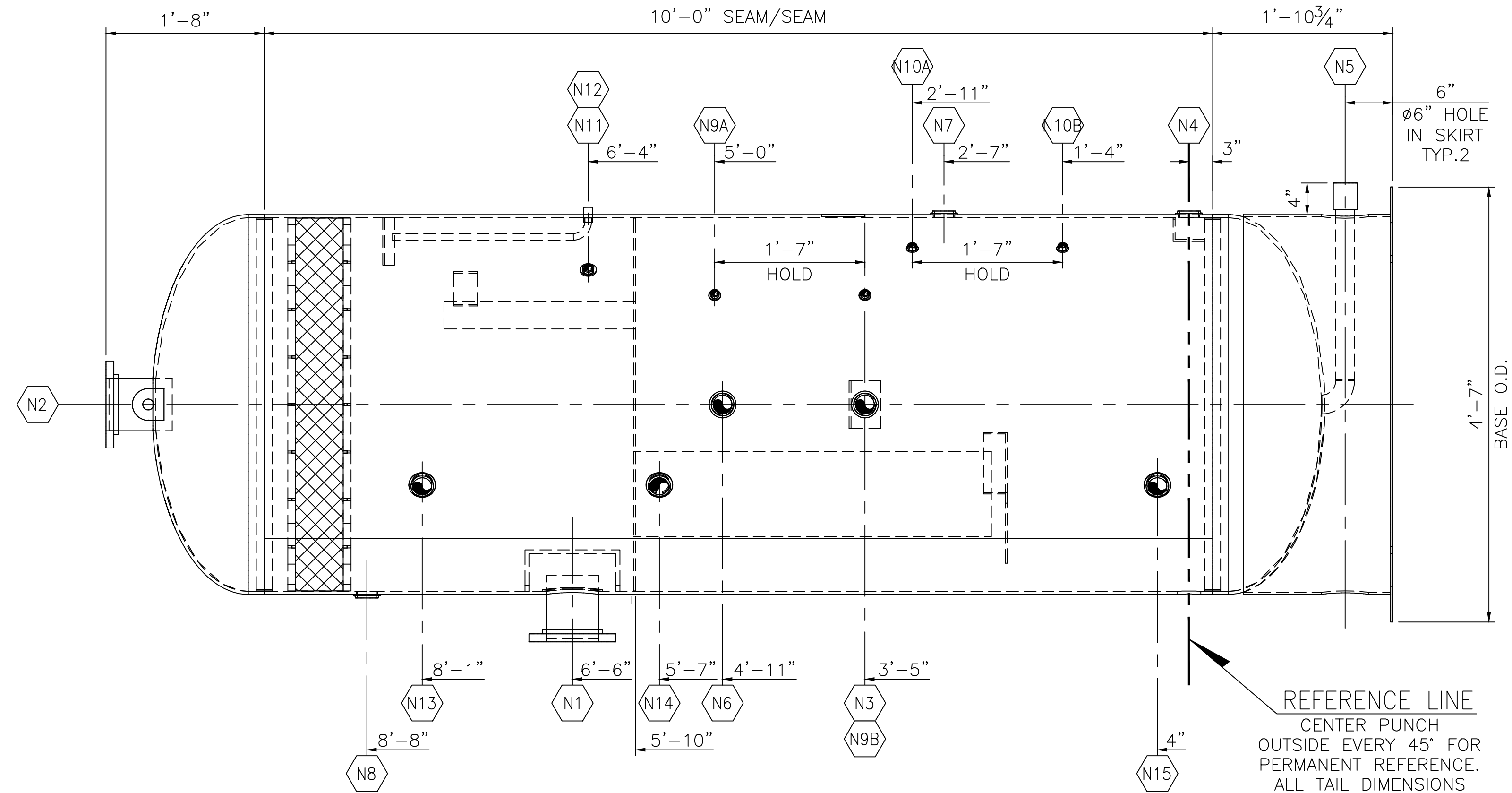
ELEVATION VIEW SCALE 1" = 1'-0"
