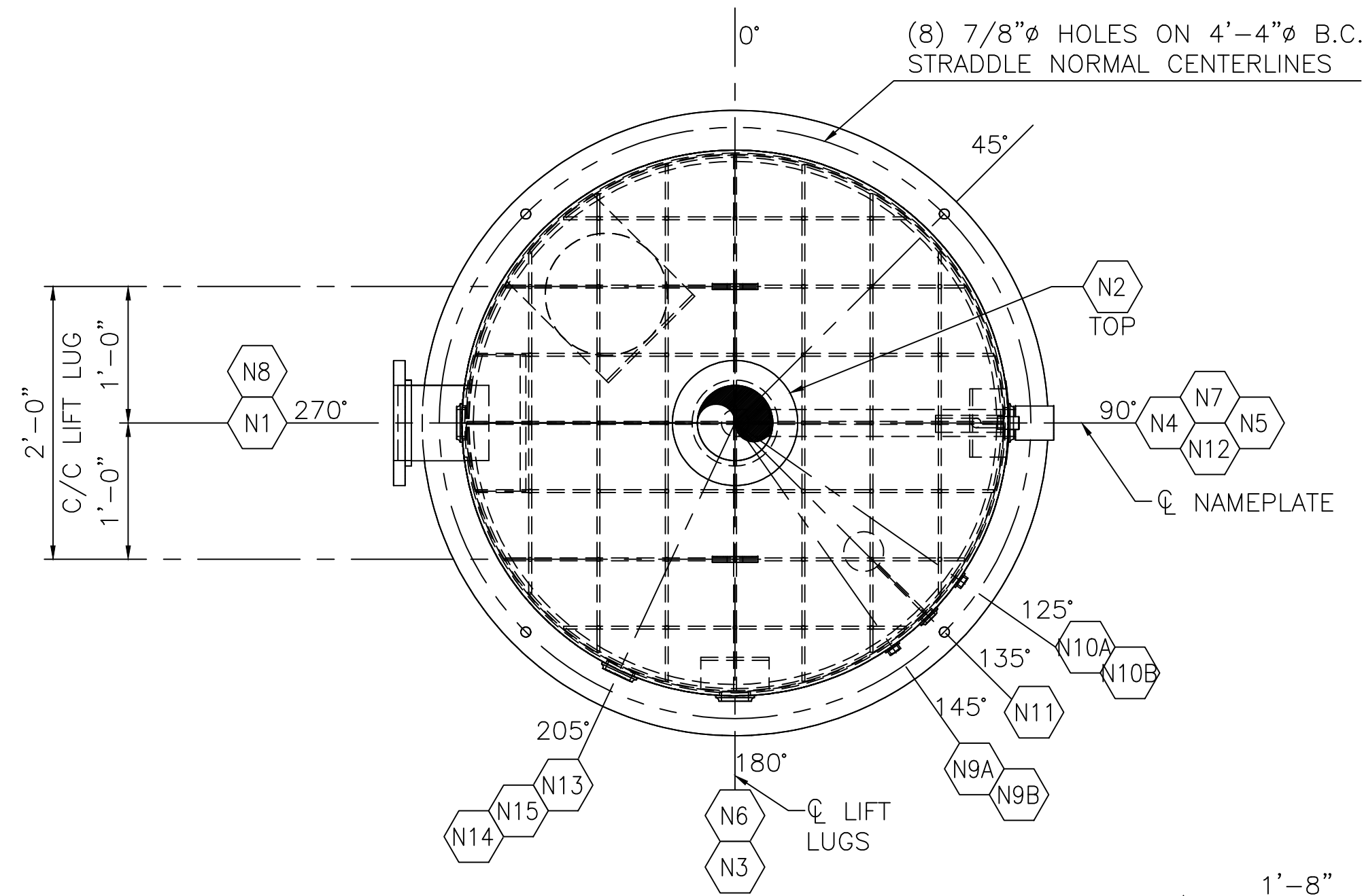
PLAN VIEW SCALE 1" = 1'-0" (TRUE ORIENTATION)
